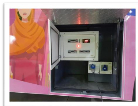
Power Distribution Box, with the option to use external single phase AC input
